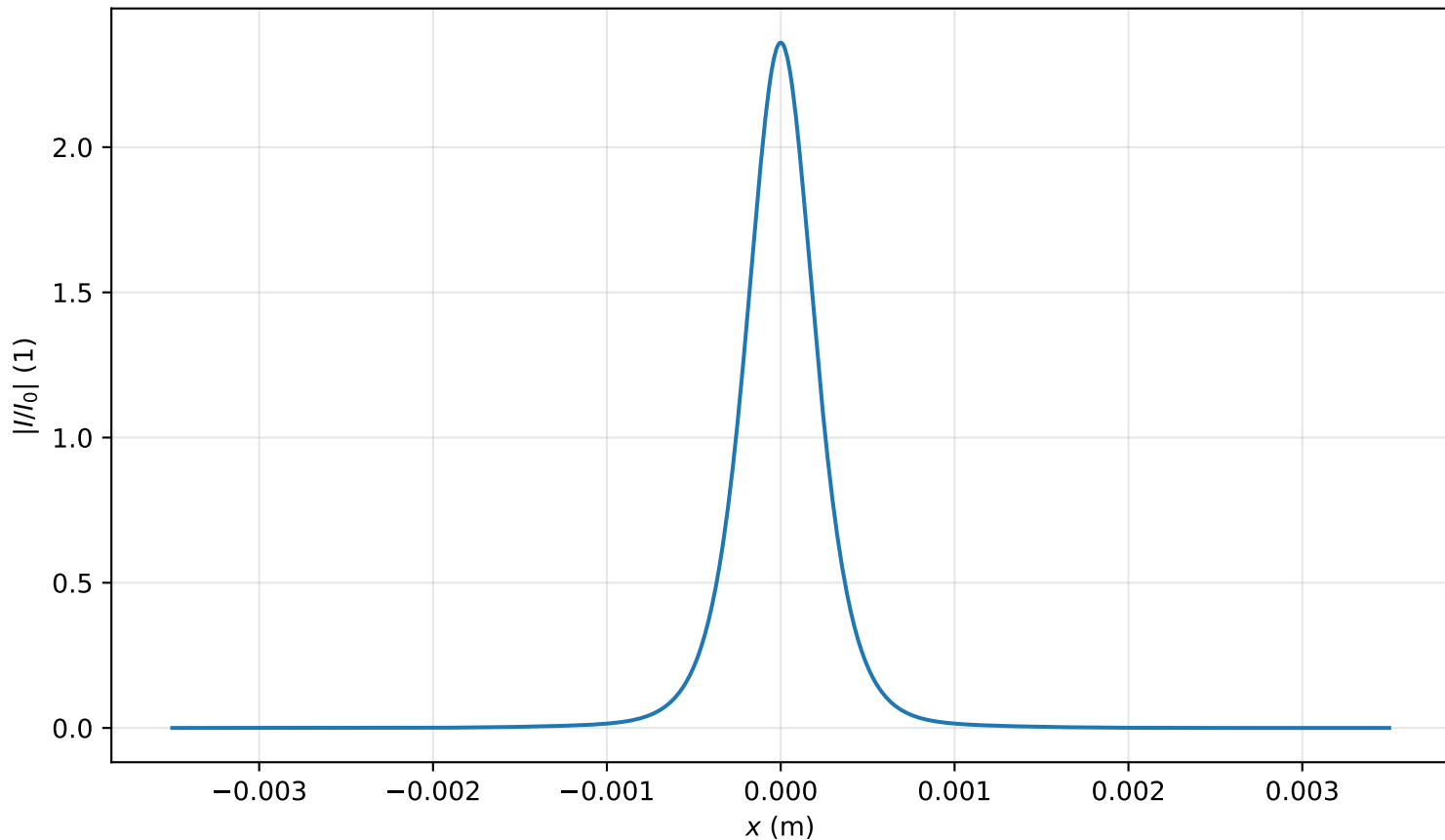
Intensity profile I(x, y = 0, z = 2.468m)/I_0 , P_{in}=1.0P_{cr} , artificial time
